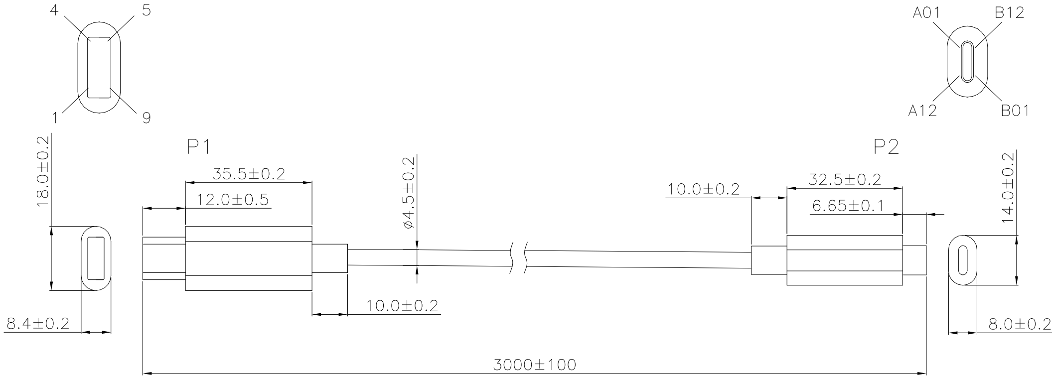
Wiring diagram
