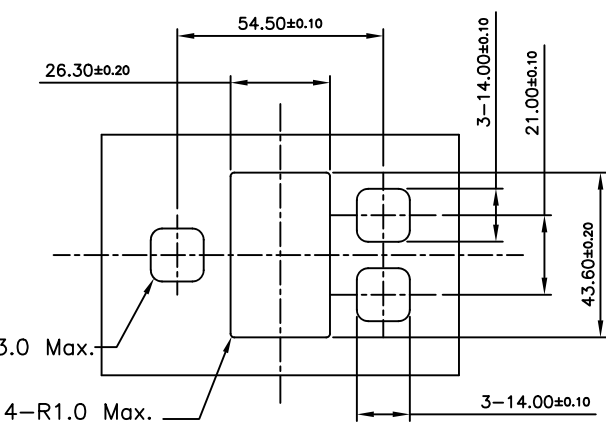
Recommended Panel Layout Pane Thickness 1.2±0.1mm
