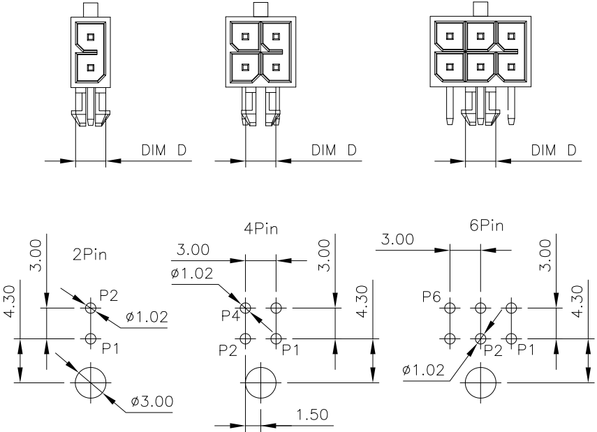
P.C.Board Layout (Top View) Tolerance: ±0.05
